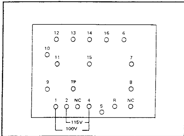
Figure 2-2. POWER TRANSFORMER TERMINALS
