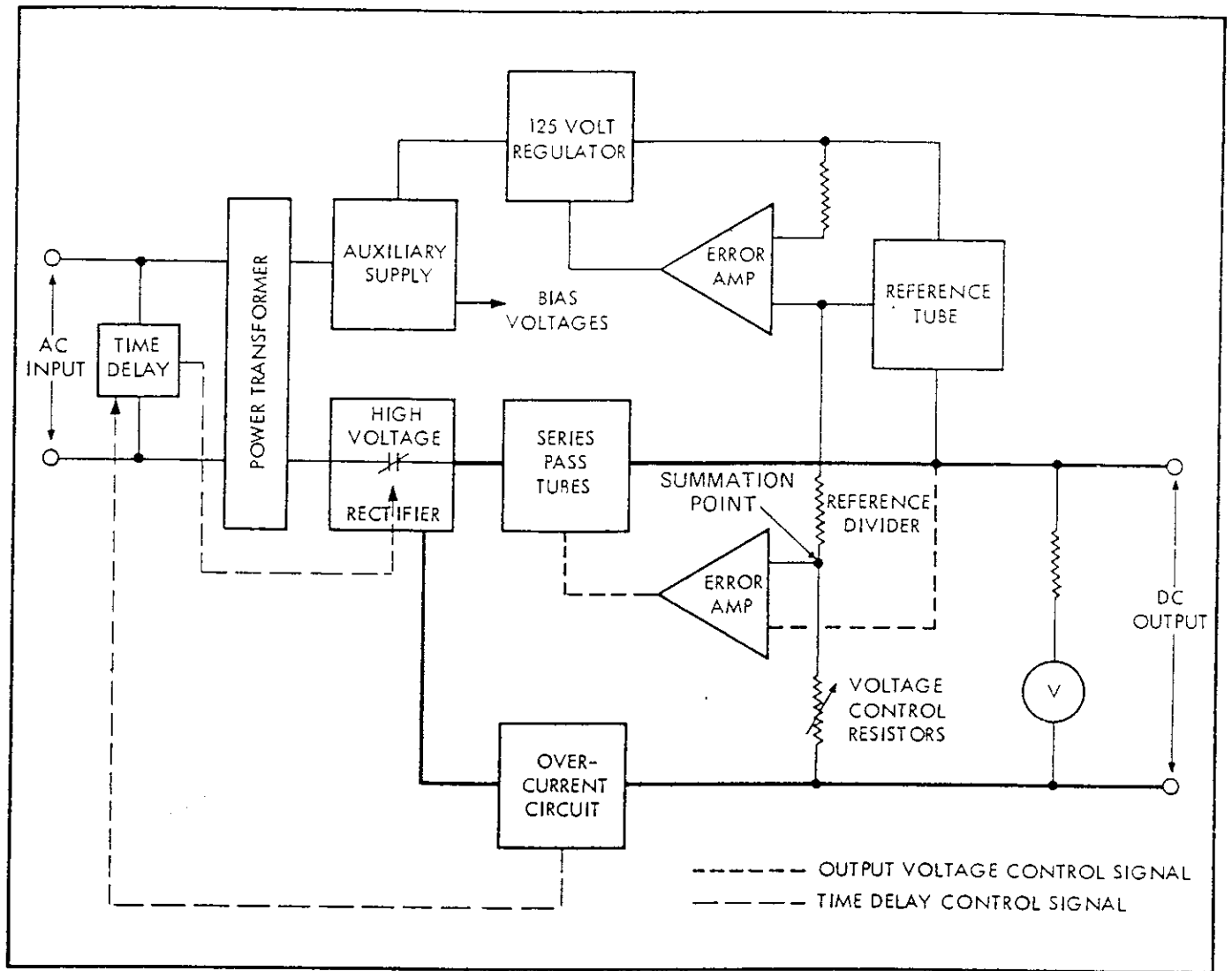
Figure 3-1. MODEL 415B BLOCK DIAGRAM
